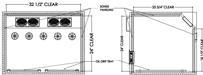
CROSS SECTION - FRONT
